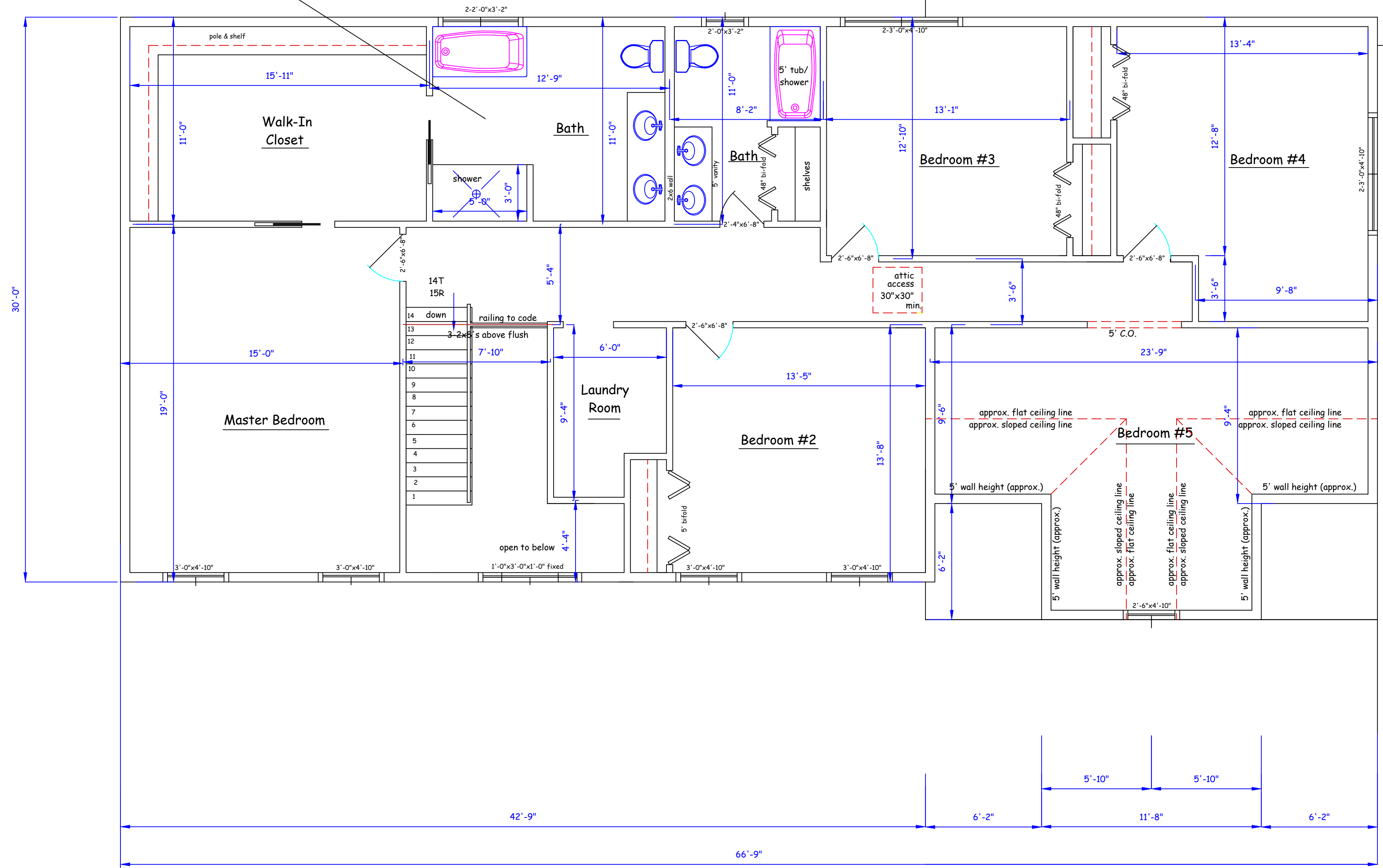
2ND. FLOOR PLAN SCALE 1/4" = 1'-0"
